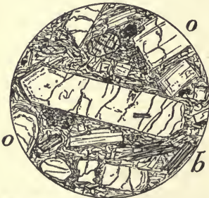
Fig. 33.—Trachyte, Ischia. \times 12 . b , Biotite. o , Orthoclase (sanidine) in fresh crystals, showing traces of zoning. Cleavages not distinct. Green soda-augite occurs; a cross-section lies near the top of the drawing. Fluidal hemicrystalline groundmass.
